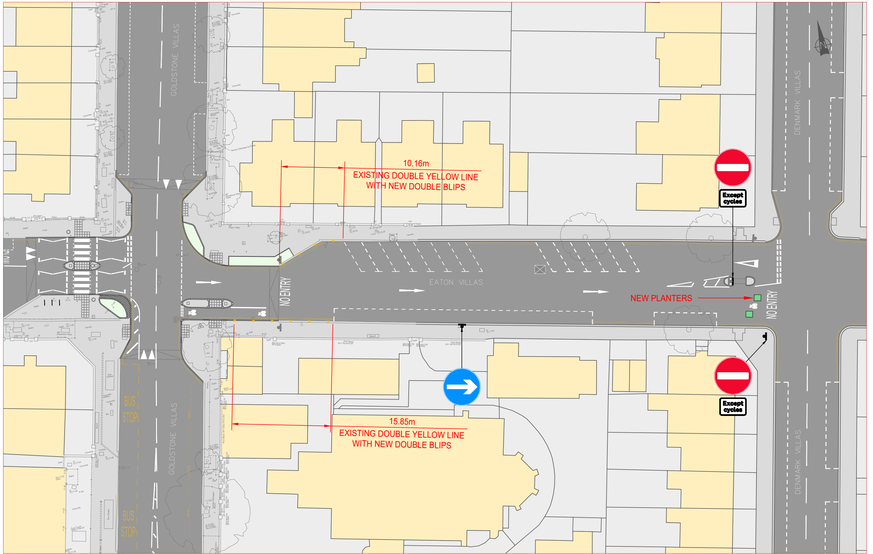
GOLDSTONE VILLAS Junction of Denmark Villas and Eaton Villas, Hove ETRO Drawing
